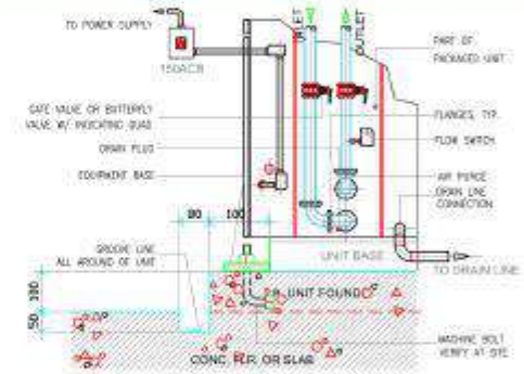
PACKAGED UNIT MOUNTING/FITTING DETAIL
