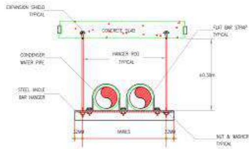
CONDENSER PIPE HANGER DETAIL
