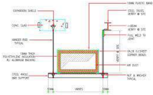
AIRDUCT HANGER DETAIL
