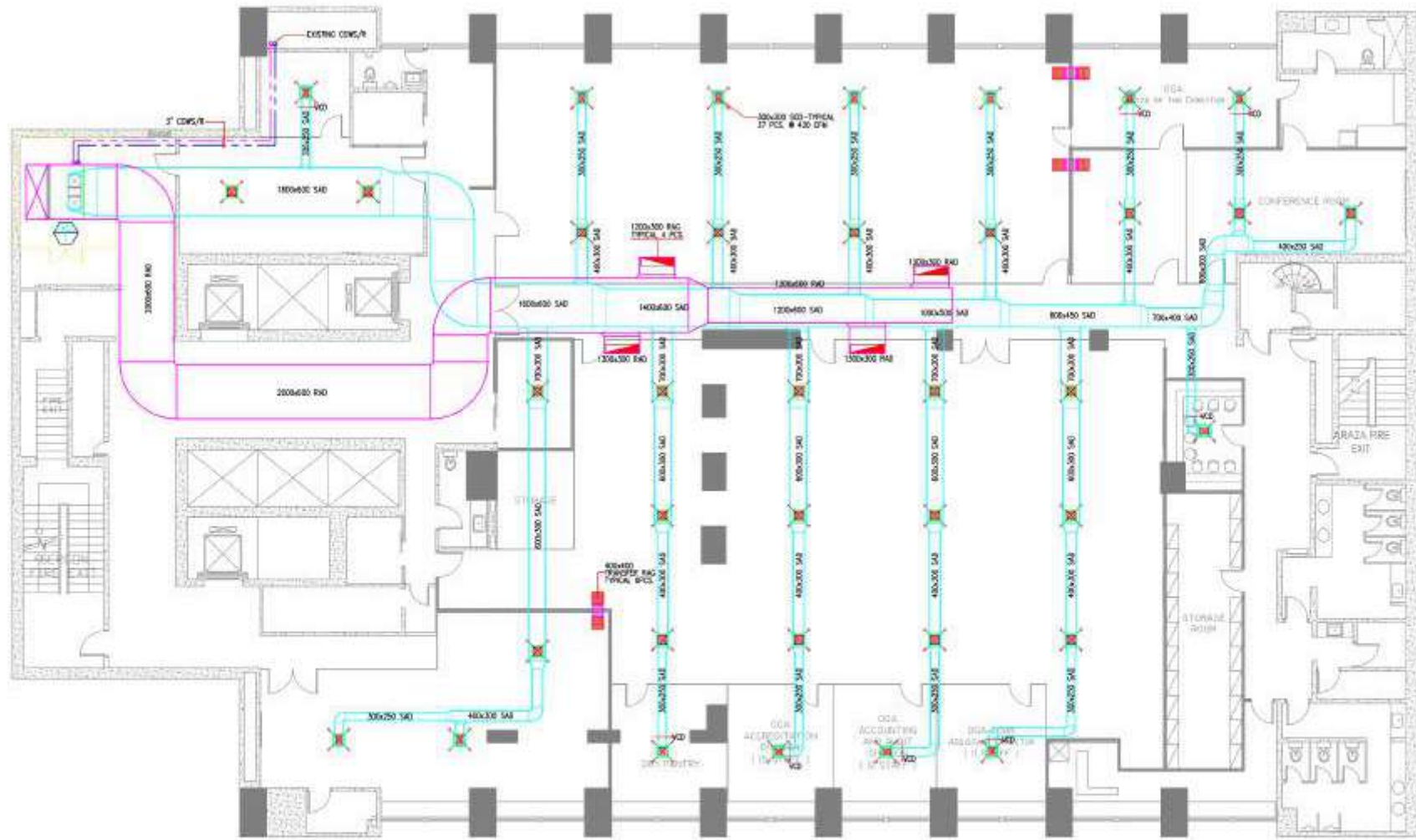
1 18TH FLOOR PROPOSED AIR CONDITIONING LAYOUT M 2 SCALE METER 1:150
